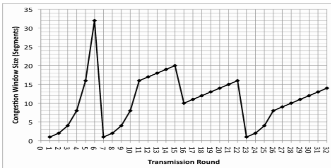
Figure 3 TCP Congestion Control
